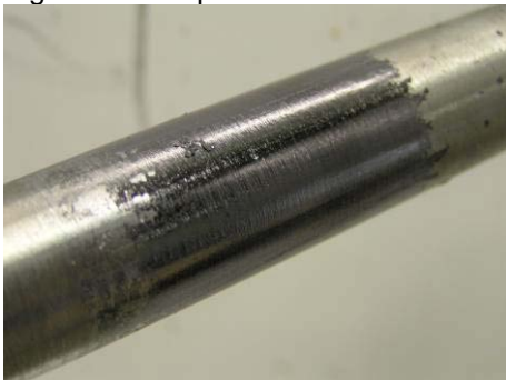
Figure 33 - 2.6 \mu mRa 35MPa
