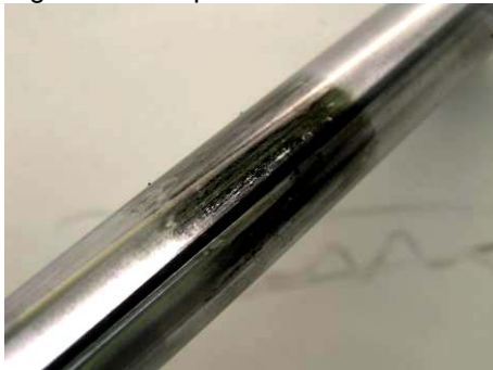
Figure 27 - 0.6μmRa 35MPa
