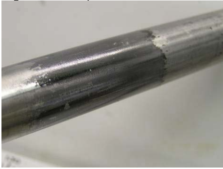
Figure 31 - 1.6 \mu mRa 35MPa
